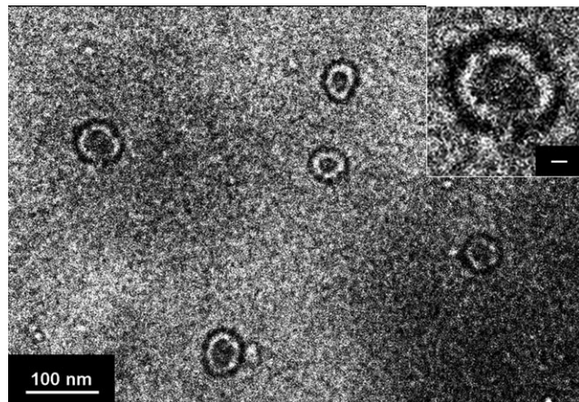
Figure 4. TEM image of an equimolar mixture of 1 and 2 from decane with concentration 5 \times 10^{-5} M and stained by RuO 4 . Inset (scale bar 10 nm) shows an enlarged view of the upper-left toroid in the main image.
